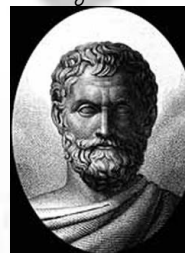
Eratosthenes
